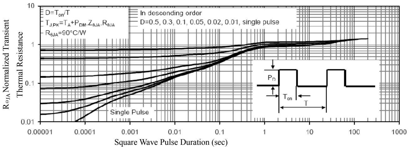
Fig.5 Normalized Maximum Effective Transient Thermal Impedance
